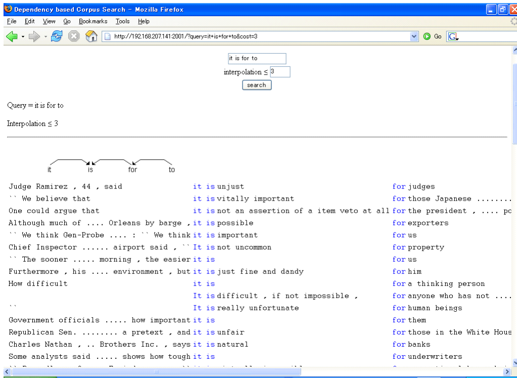
Fig. 6. A screen shot of the system
