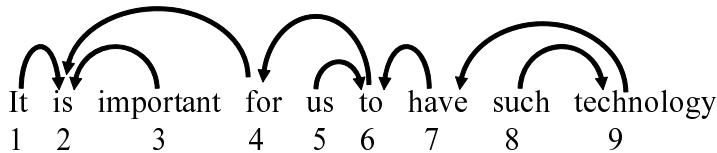
Fig. 4. Dependencies for “It is important for us to have such technology”
