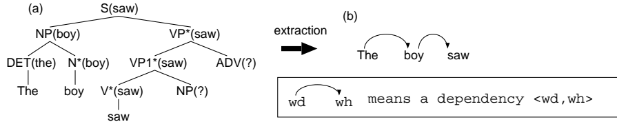
Figure 3: An example of computing dependencies for initial fragments
