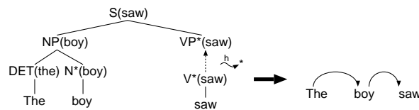
Figure 5: An example of propagation of head-word
